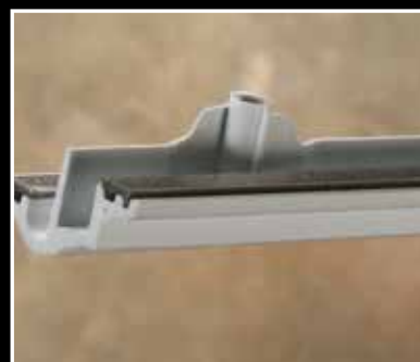
Full rib integrated with screw boss for enhanced strength.
