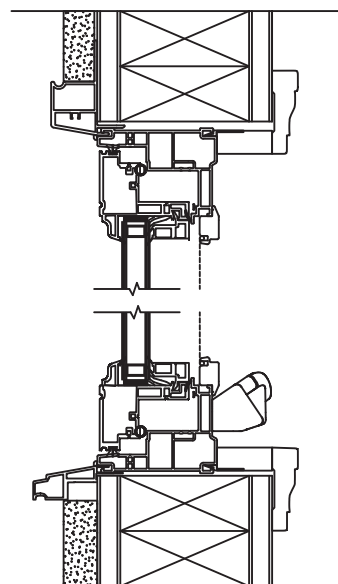
Trinity® Casement Full Frame Installation
