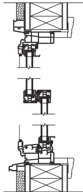
Trinity® Double Hung Full Frame Installation
